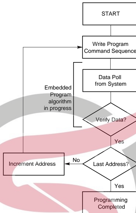
Figure 10.1 Program Operation
