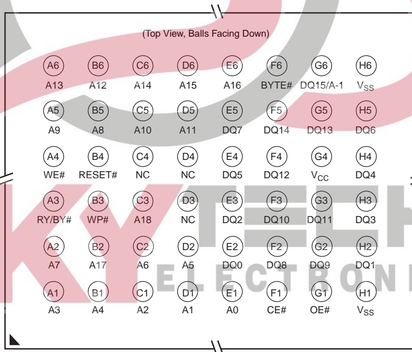
Figure 3.2 48-ball Fine-pitch BGA (VBK048)
